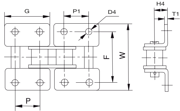
Attachment 90° 2 sides 2 holes
