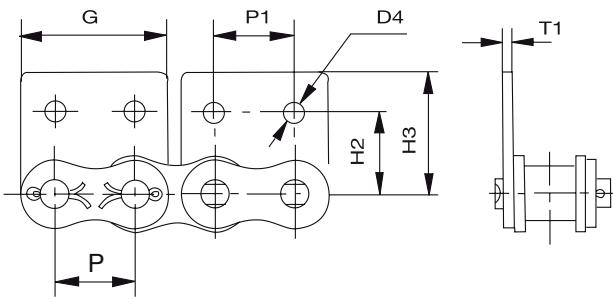
Straight attachment 1 side 2 holes WSA-2
