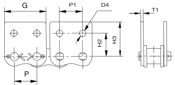
Straight attachment 2 sides 2 holes WSK-2
